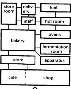
5 Functional diagram for a bakery: good ventilation needed, possibly dehumidify
